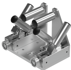
V20 ADJ. Roller Part No. 00009MC220
